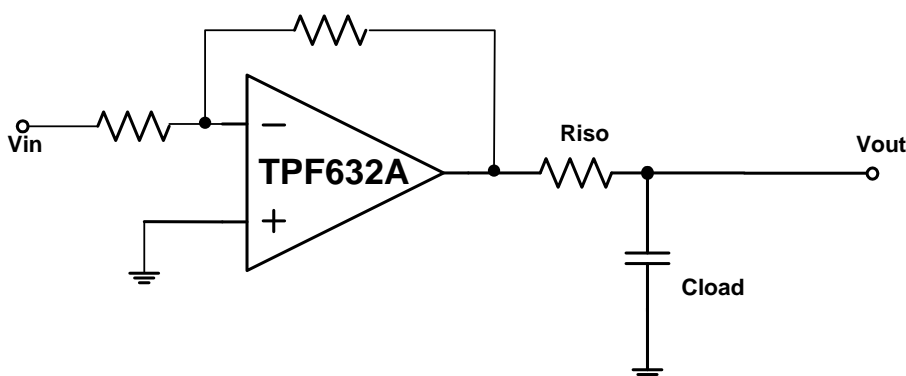
Figure 8 Driving Circuits
