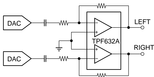
Figure 1. Typical Application Circuit of TPF632A
