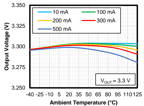
Figure 6 Output Voltage vs. Temperature
