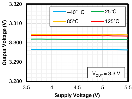
Figure 3 Line Regulation
