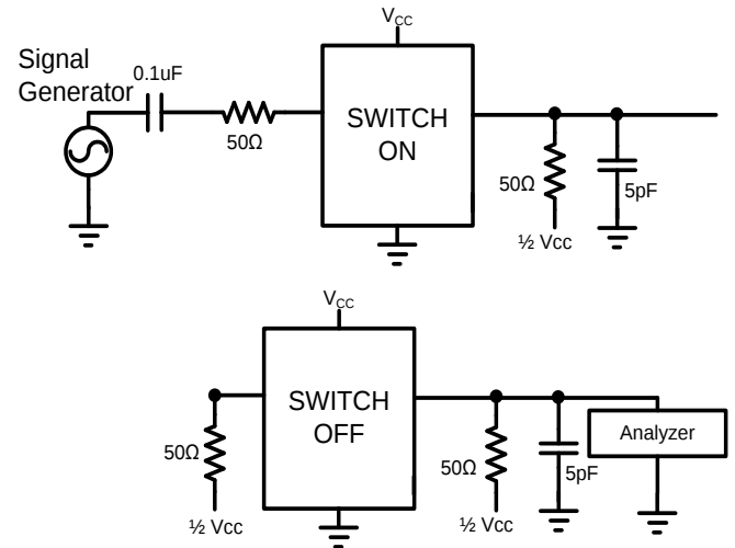
Figure 9 Crosstalk
